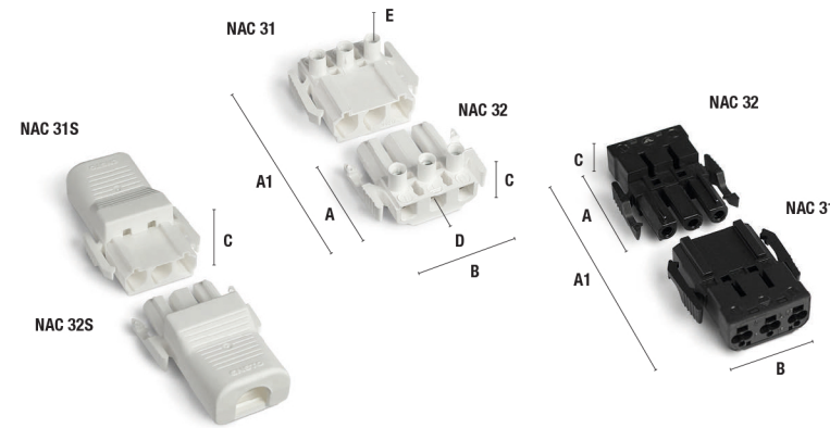
Legenda delle quote Legend for dimensions
