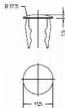
Lens dimensions
