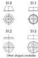
Lens dimensions
